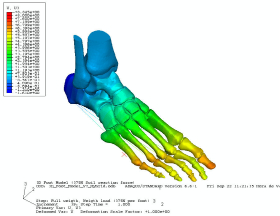
Fig. 18 – Nodal displacement (Pure Compression)
