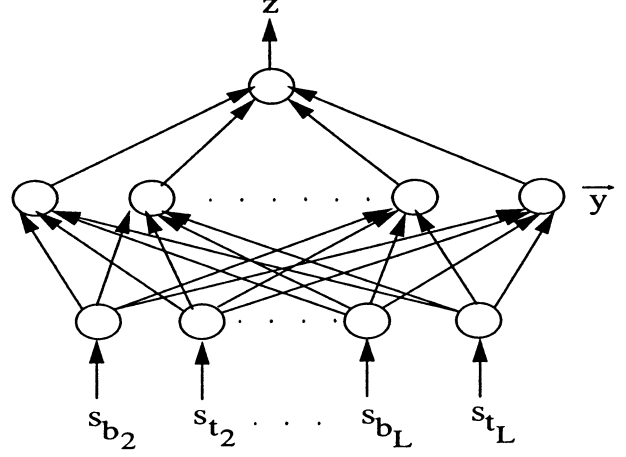
Fig. 4. Multilayer perceptron
