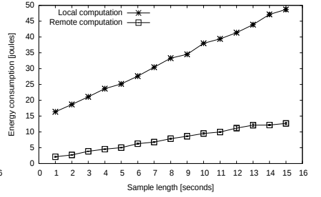
Figure 6. Speaker recognition energy consumption vs audio sample length.
