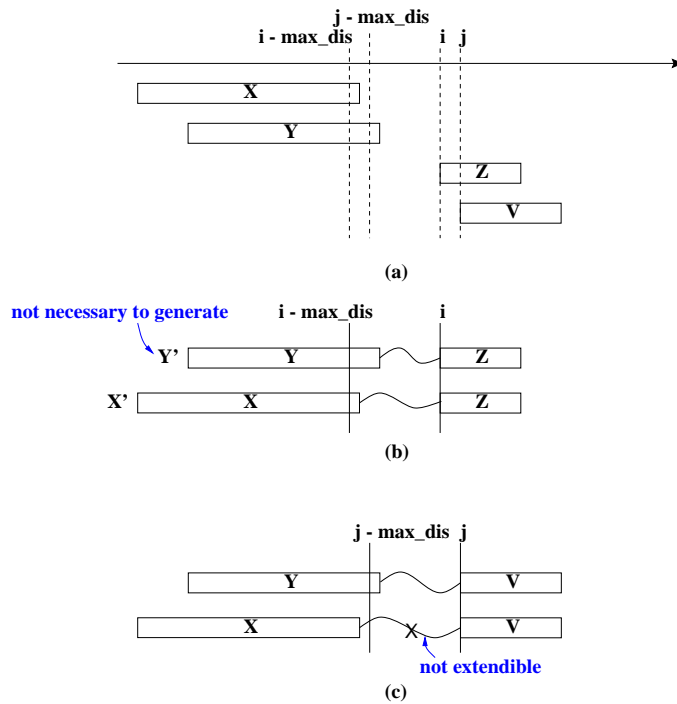
Figure 4: Subsequence Dominance
