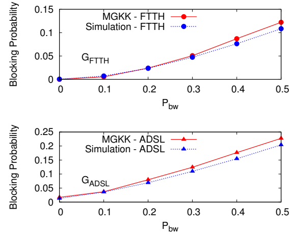
Fig. 5. Comparison of the blocking probability between analytical model M/G/K/K and simulation results when increasing the bandwidth heterogeneity in the system P_{bw} . System load \rho = 0.9 has been considered for both G_{FTTH} (top) and G_{ADSL} (bottom) scenarios.
