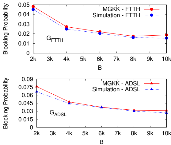
Fig. 7. Comparison of the blocking probability between analytical model M/G/K/K and simulation results when increasing the number of STBs in the system for both G_{FTTH} (top) and G_{ADSL} (bottom) scenarios. System load \rho = 1.0 .
